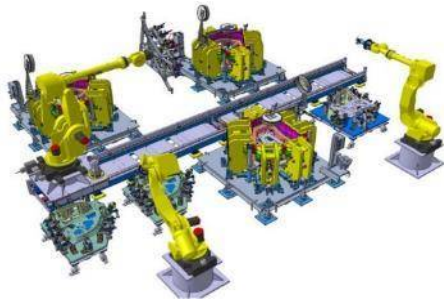
Automotive Body-In-White & Chassis Assembly System
