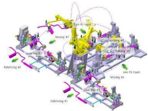
Automated Welding Assembly Lines
